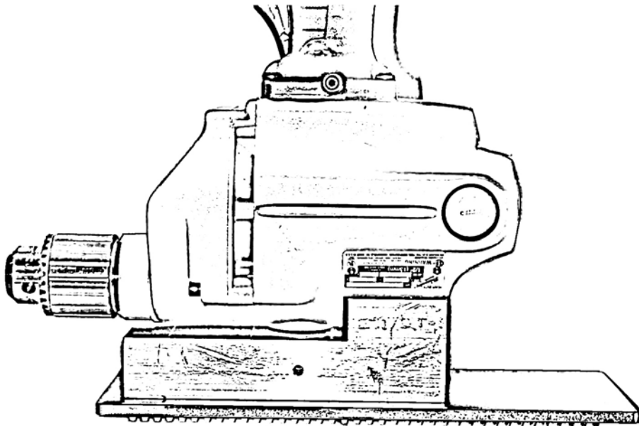
Uni-Block, TD-2 (traverse plate) & Drill Mounted together as one piece
